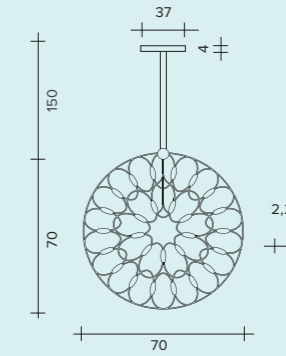
LED 27W - 24V 2700°K / 2025 lumen 3000°K / 2160 lumen
