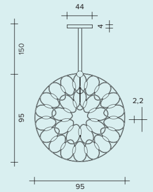
LED 54W - 24V 2700°K / 4050 lumen 3000°K / 4320 lumen
